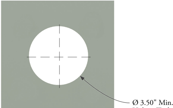
Figure 20 Fuseholder Mounting Dimensions
