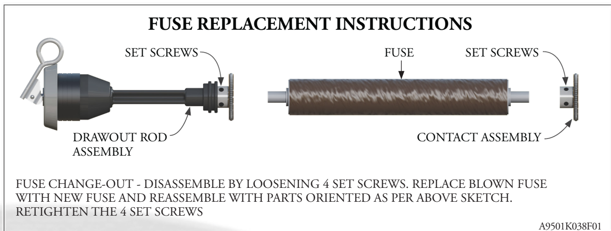
Figure 19 Decal (Submersible-Non-Loadbreak)
