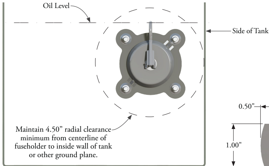
Figure 17 General Fuseholder Application (See Figure 21 for Vertical Mounting)
