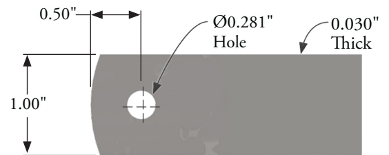
Figure 18 Detail of Terminal
