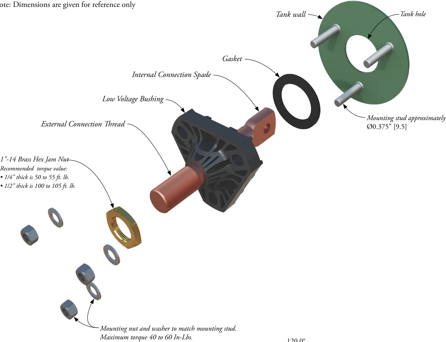
Figure 1 Mounting
